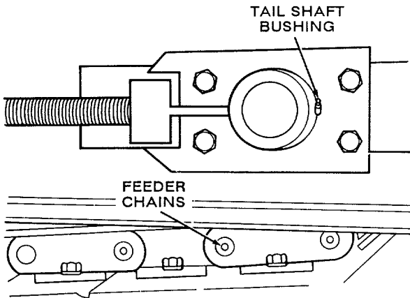
(C) Feeder Chains and Tail Shaft Bushing
