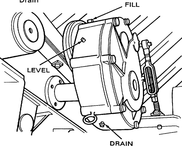
R Feeder Shaft Gear Reducer Fill, Level, and Drain
