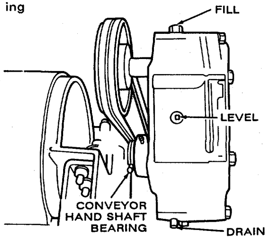
W Conveyor Shaft Gear Reducer Fill, Level, and Drain, and Conveyor Head Shaft Bearing
